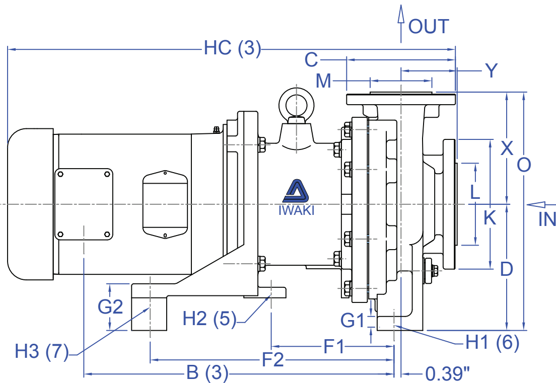
PUMP DIMENSIONS (1)
