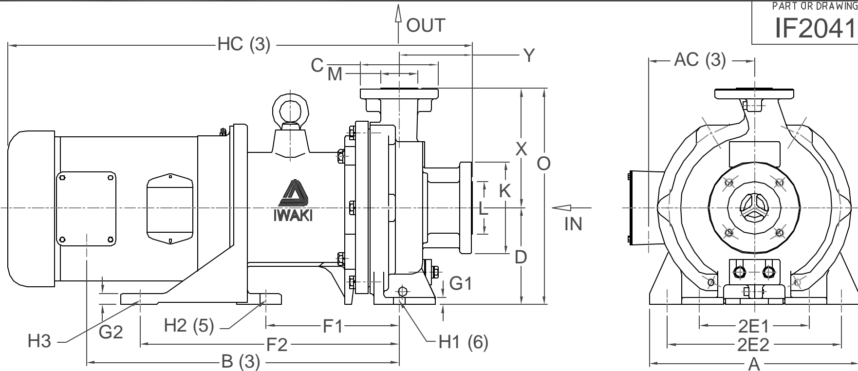
PUMP DIMENSIONS (1)
